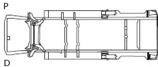
UNDERBODY VIEW
